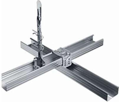
HANGER PLATE
